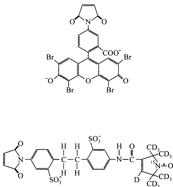
FIGURE 1 Chemical structures of eosin-5-maleimide ( top ) and [ ^{15}\text{N} , ^2\text{H}_{13} ]-SL-H 2 -DADS-maleimide ( bottom ).
