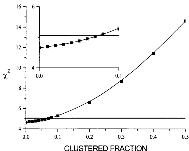
FIGURE 9 Effect of a highly clustered fraction of band 3 on fitting experimental ST-EPR data. The experimental ST-EPR spectra from control ghosts obtained at X- and Q-band microwave frequencies (upper row of Fig. 5) were simultaneously fit to a two-component model where one component exhibited unconstrained URD and the second component was immobilized on the ST-EPR timescale ( \tau = 10 ms). The \chi^2 values on the ordinate represent the best fits of this two-component model that were obtained by allowing the correlation time for the unrestricted component to float in the calculation. The solid horizontal line is the 95% confidence level for discriminating between this two-component model and a single unrestricted URD model.
