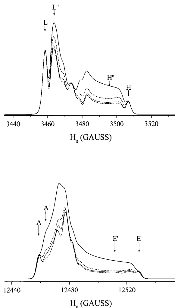
FIGURE 3 Calculated V_2' ST-EPR spectra at X-band (top) and at Q-band (bottom) for a restricted amplitude URD model. Each panel shows spectra calculated for \Delta = 1^\circ (solid line), \Delta = 30^\circ (dashed line), \Delta = 60^\circ (short dashed line), and \Delta = 90^\circ (dot-dash line). The spectra were calculated at 50-kHz Zeeman field modulation frequency, \tau = 15 \mu\text{s} , \theta = 37^\circ , and \phi = 61^\circ using a microwave observer field of 0.2 Gauss. The field positions where spectral amplitudes that are sensitive to \Delta are measured are shown superimposed on the calculated spectra at X- and Q-band.
